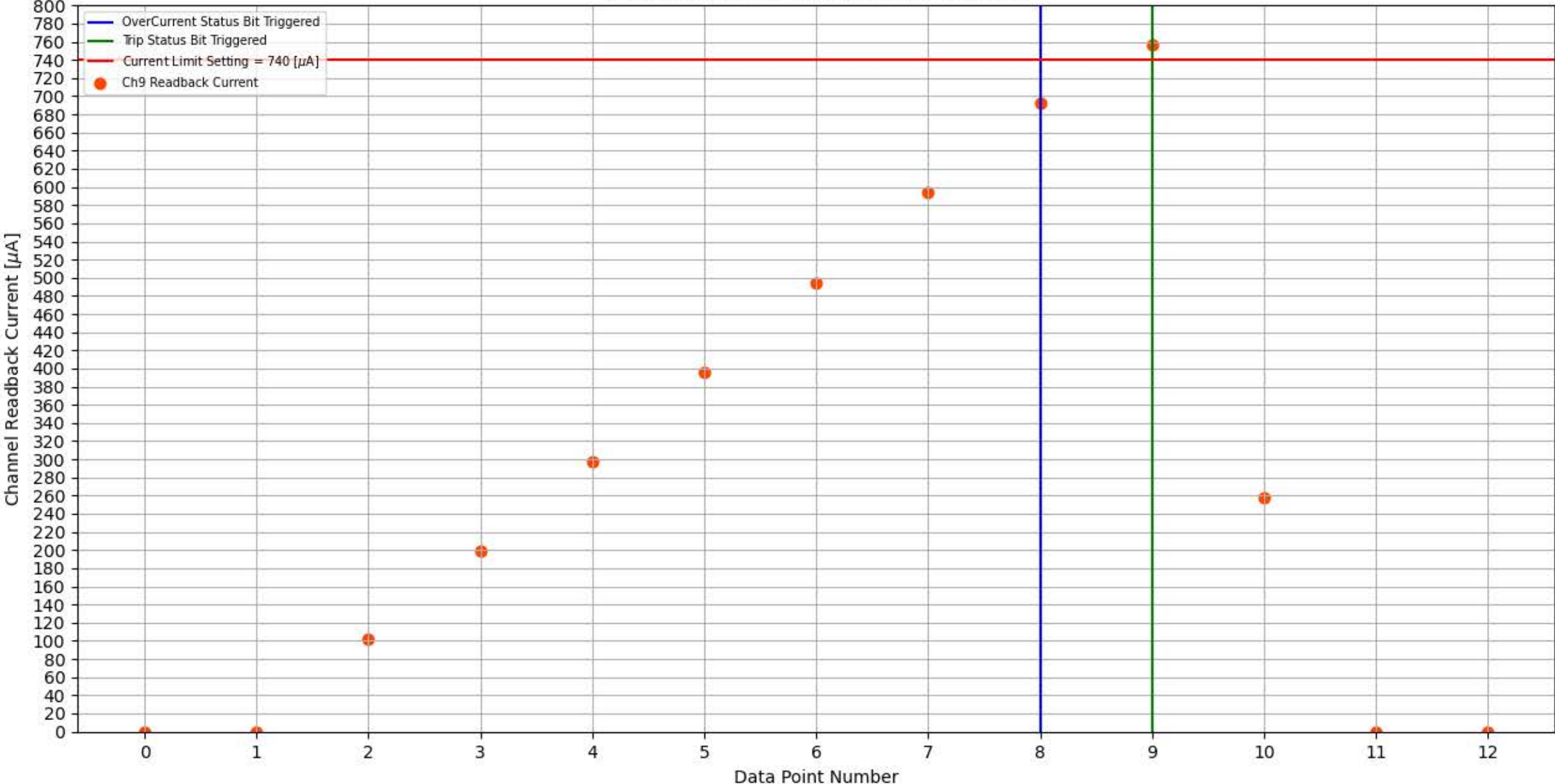
Module 350, Slot 13, Channel 9 Trip Test
