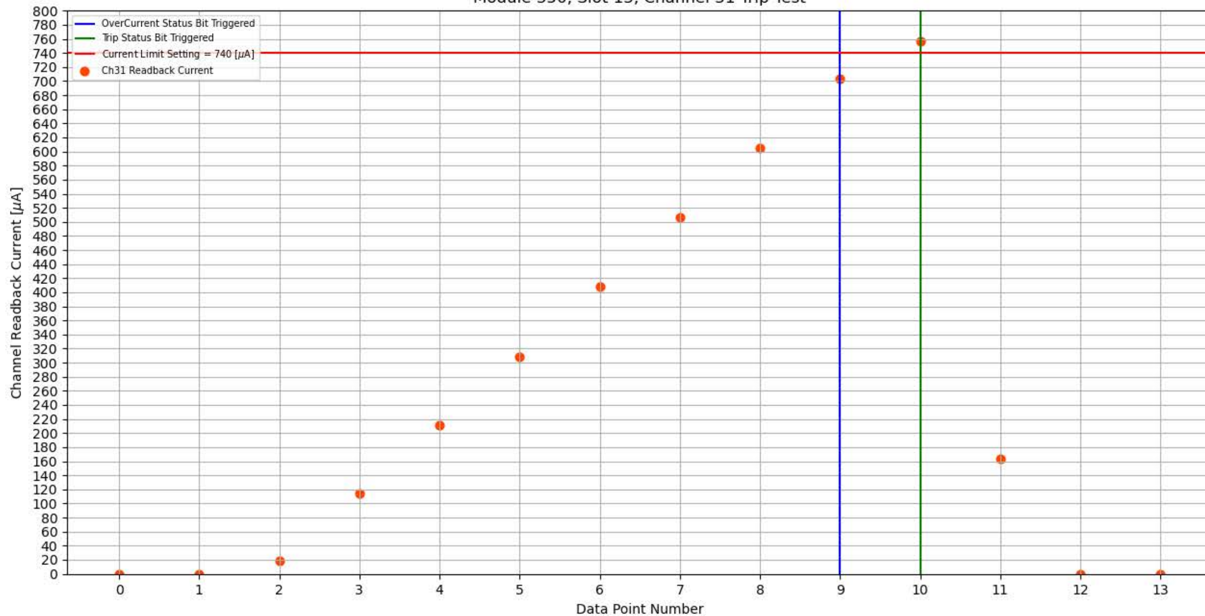
Module 350, Slot 13, Channel 31 Trip Test
