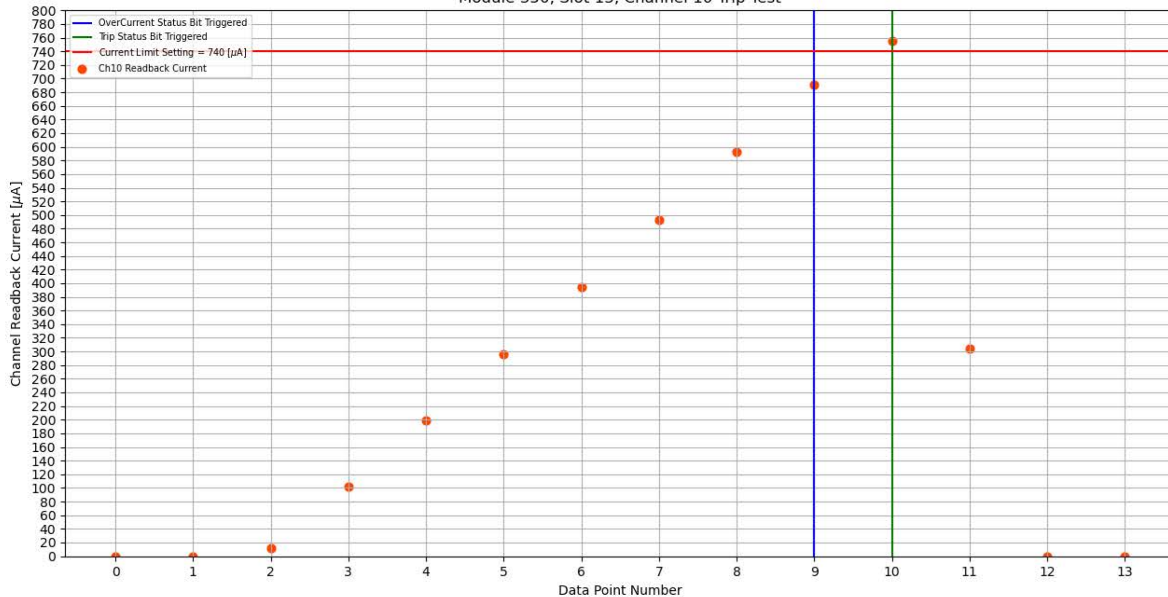
Module 350, Slot 13, Channel 10 Trip Test
