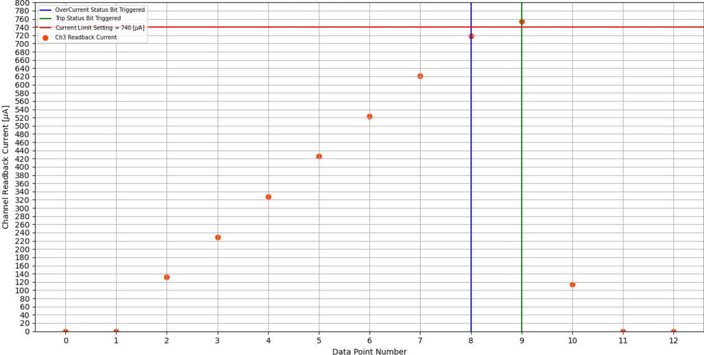
Module 350, Slot 13, Channel 3 Trip Test
