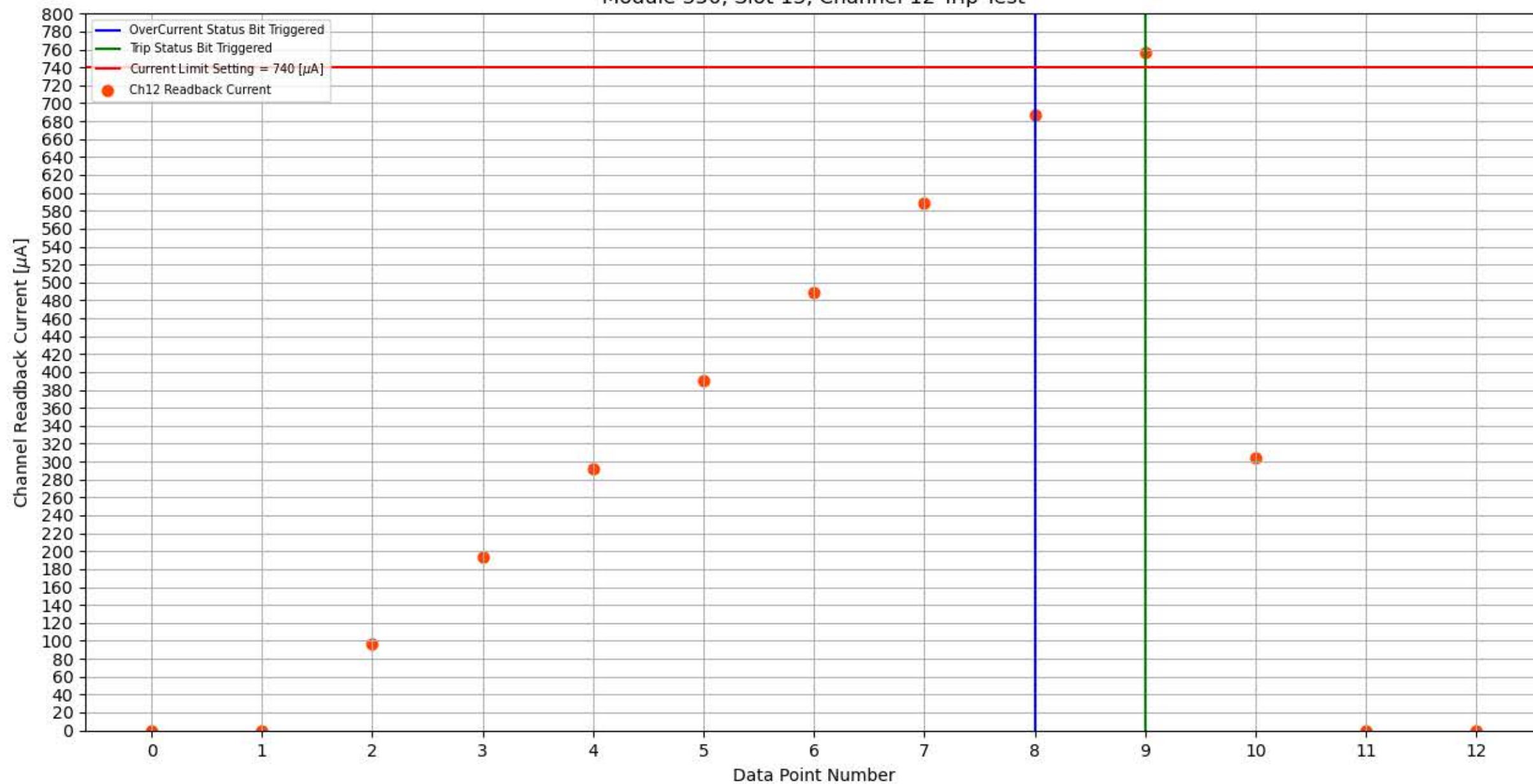
Module 350, Slot 13, Channel 12 Trip Test
