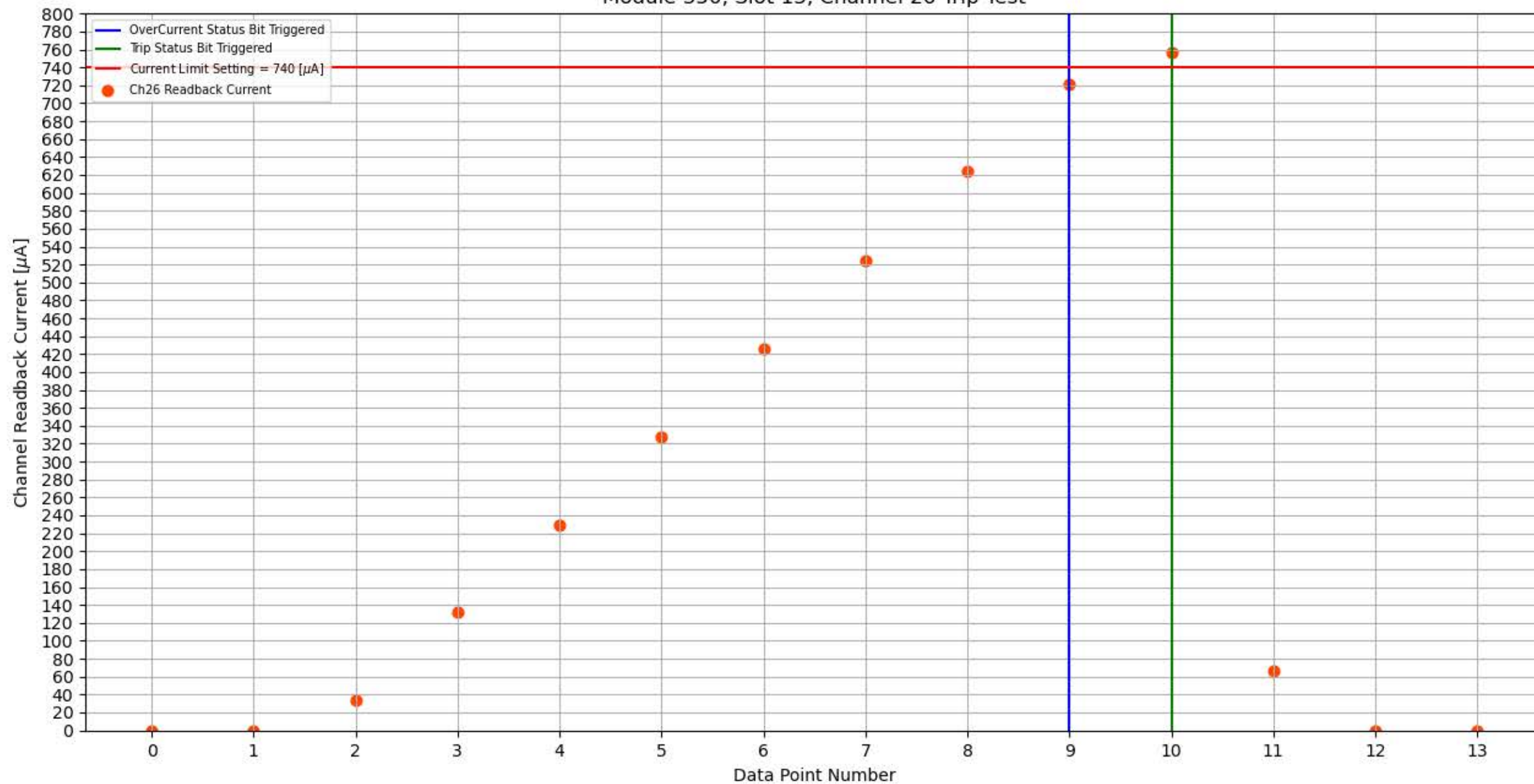
Module 350, Slot 13, Channel 26 Trip Test
