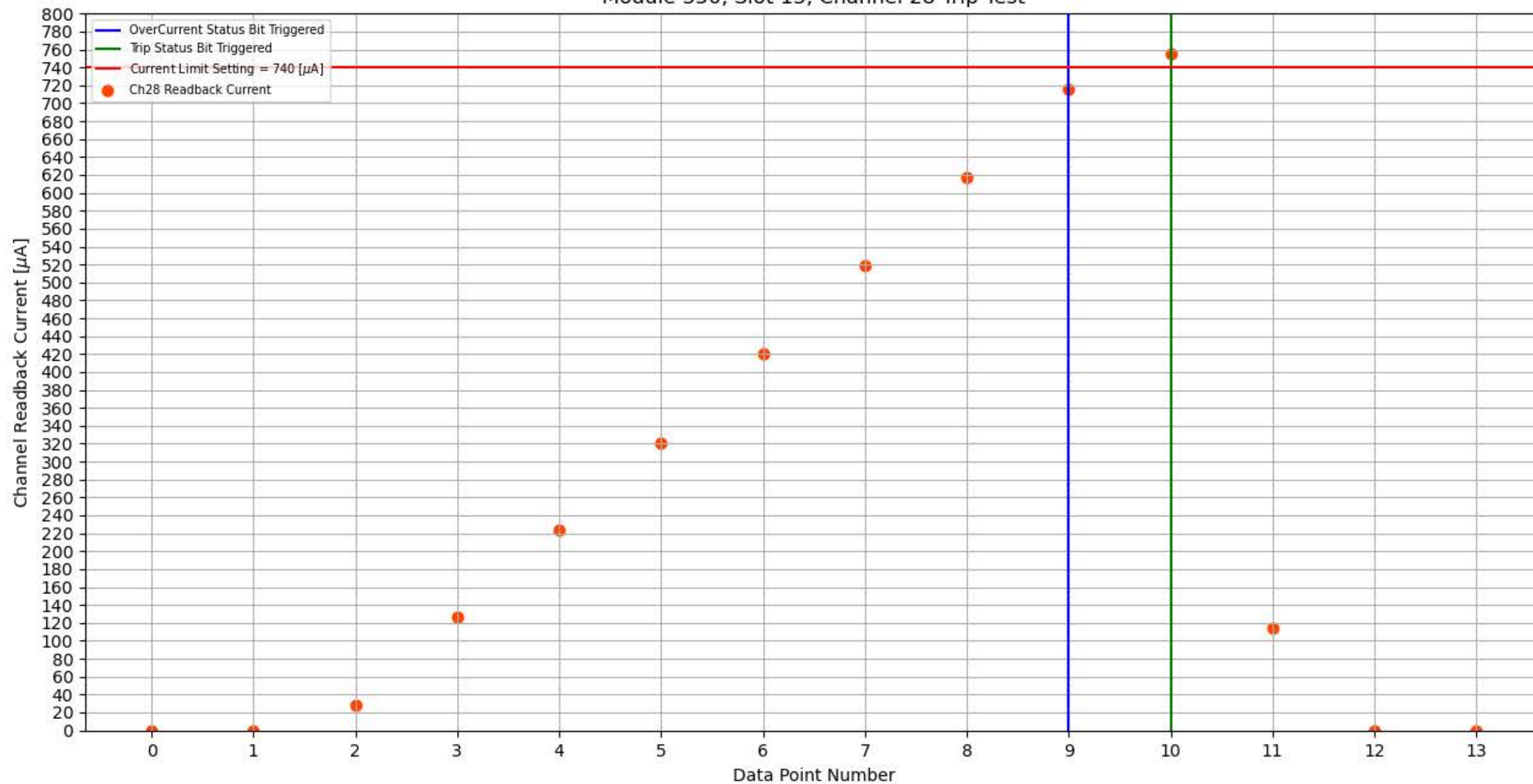
Module 350, Slot 13, Channel 28 Trip Test
