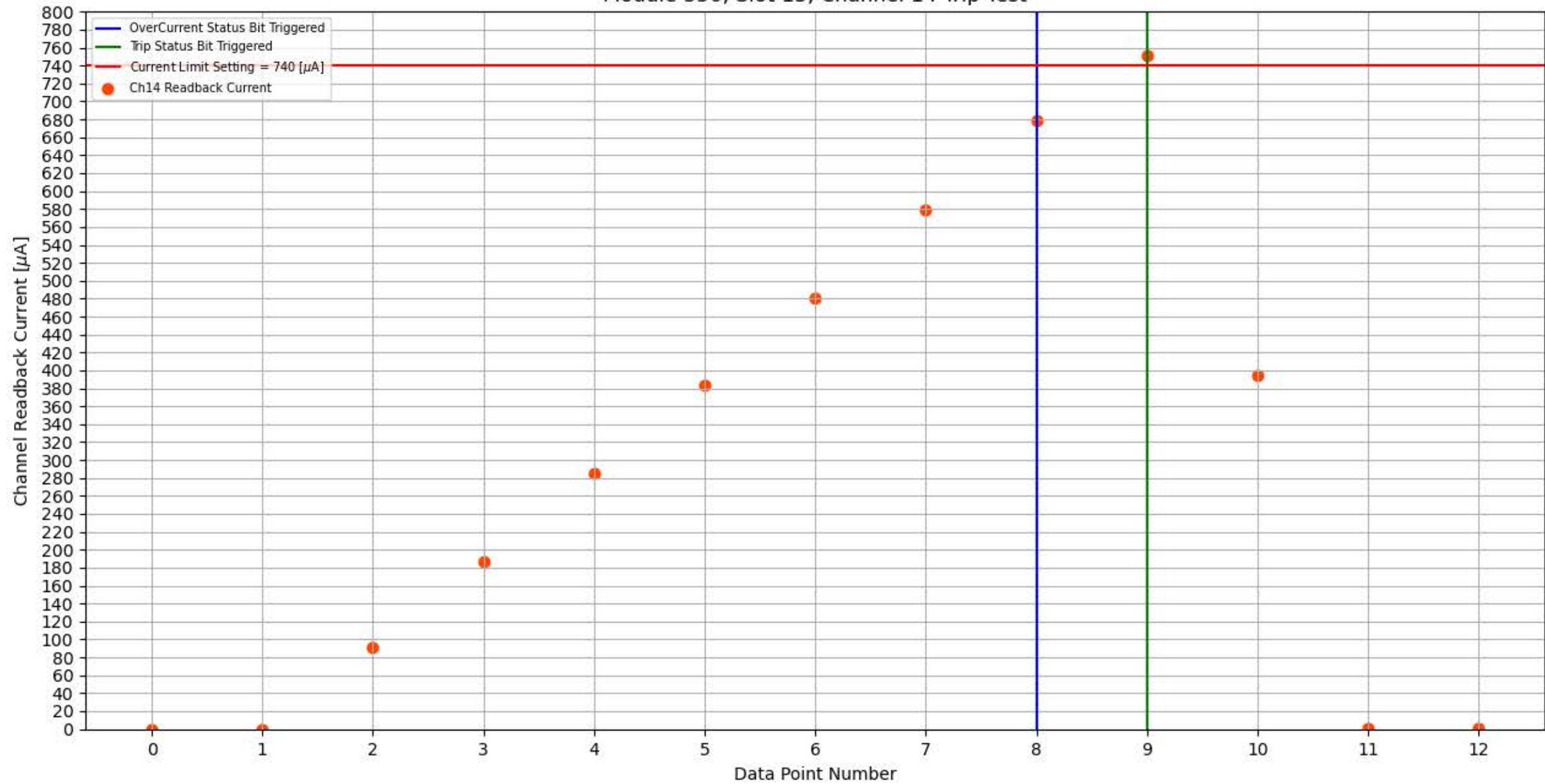
Module 350, Slot 13, Channel 14 Trip Test
