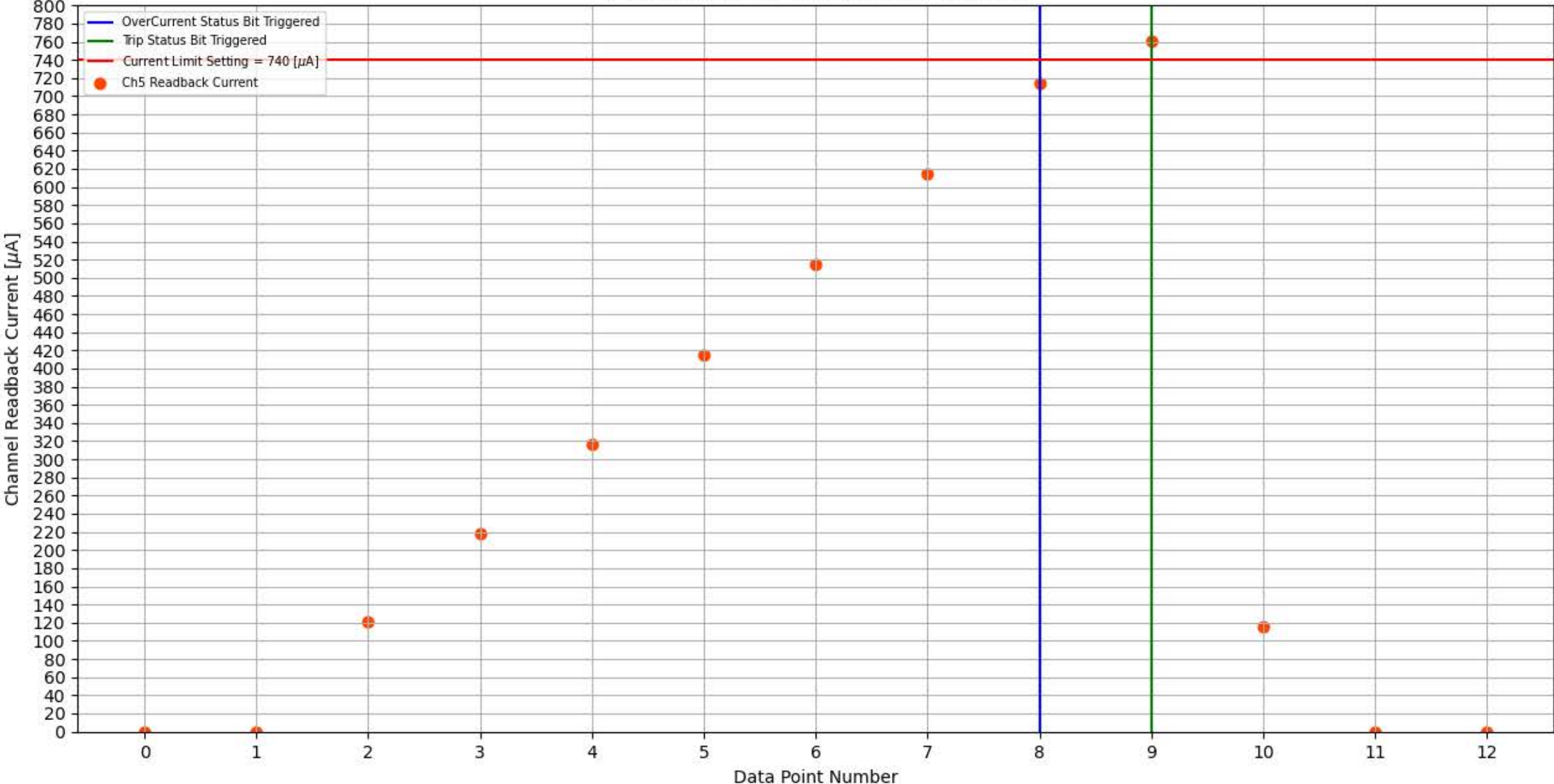
Module 350, Slot 13, Channel 5 Trip Test
