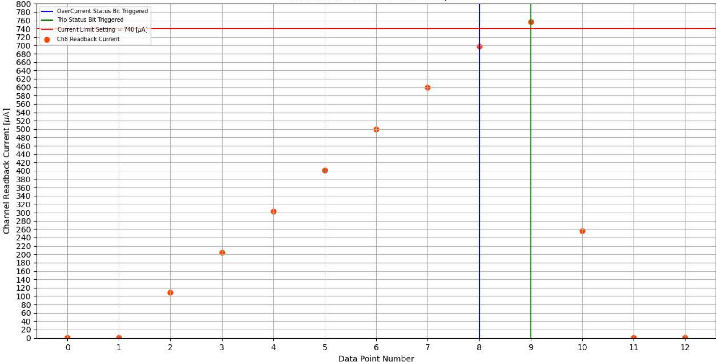
Module 350, Slot 13, Channel 8 Trip Test
