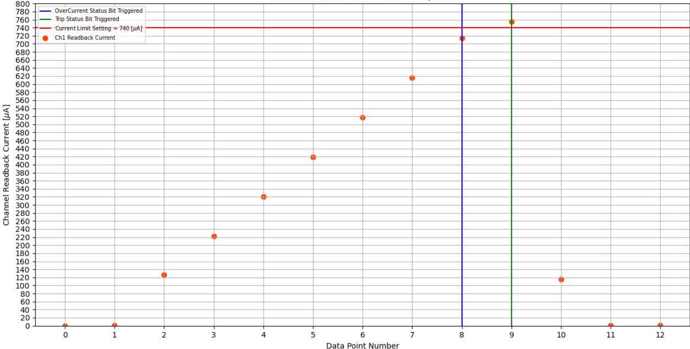
Module 350, Slot 13, Channel 1 Trip Test
