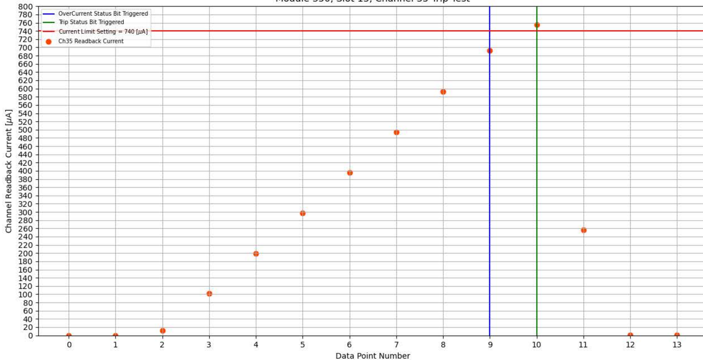
Module 350, Slot 13, Channel 35 Trip Test
