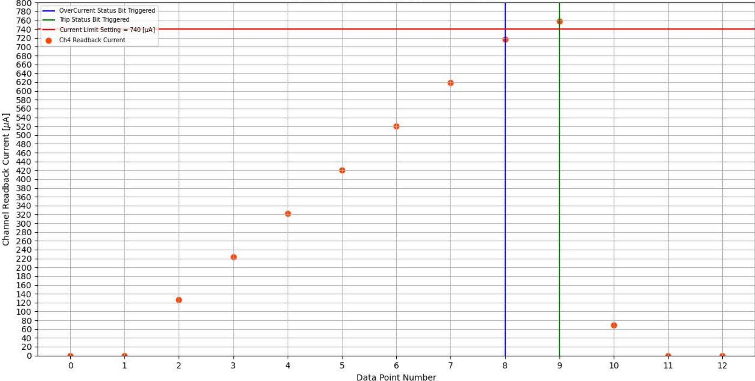
Module 350, Slot 13, Channel 4 Trip Test
