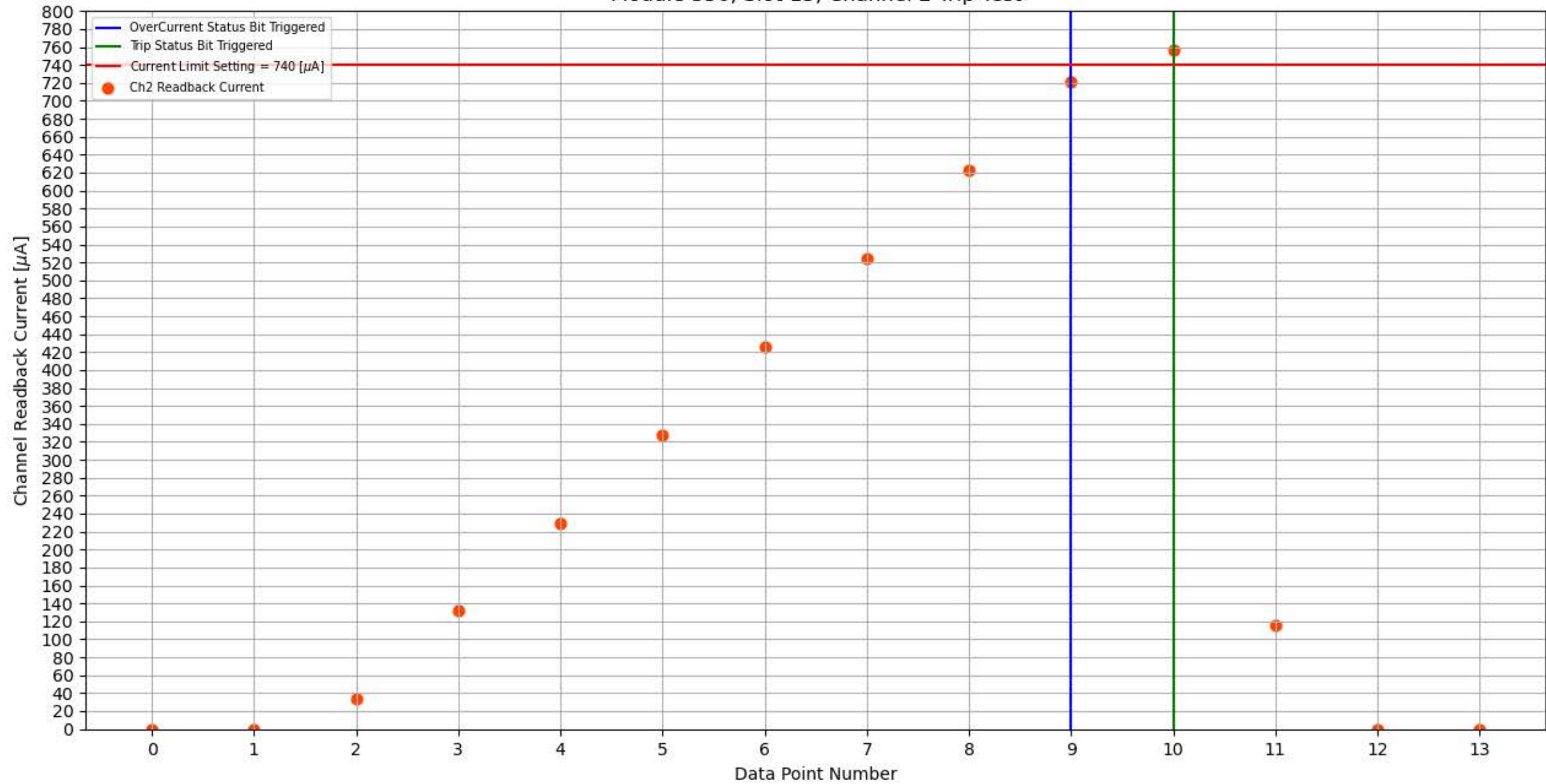
Module 350, Slot 13, Channel 2 Trip Test
