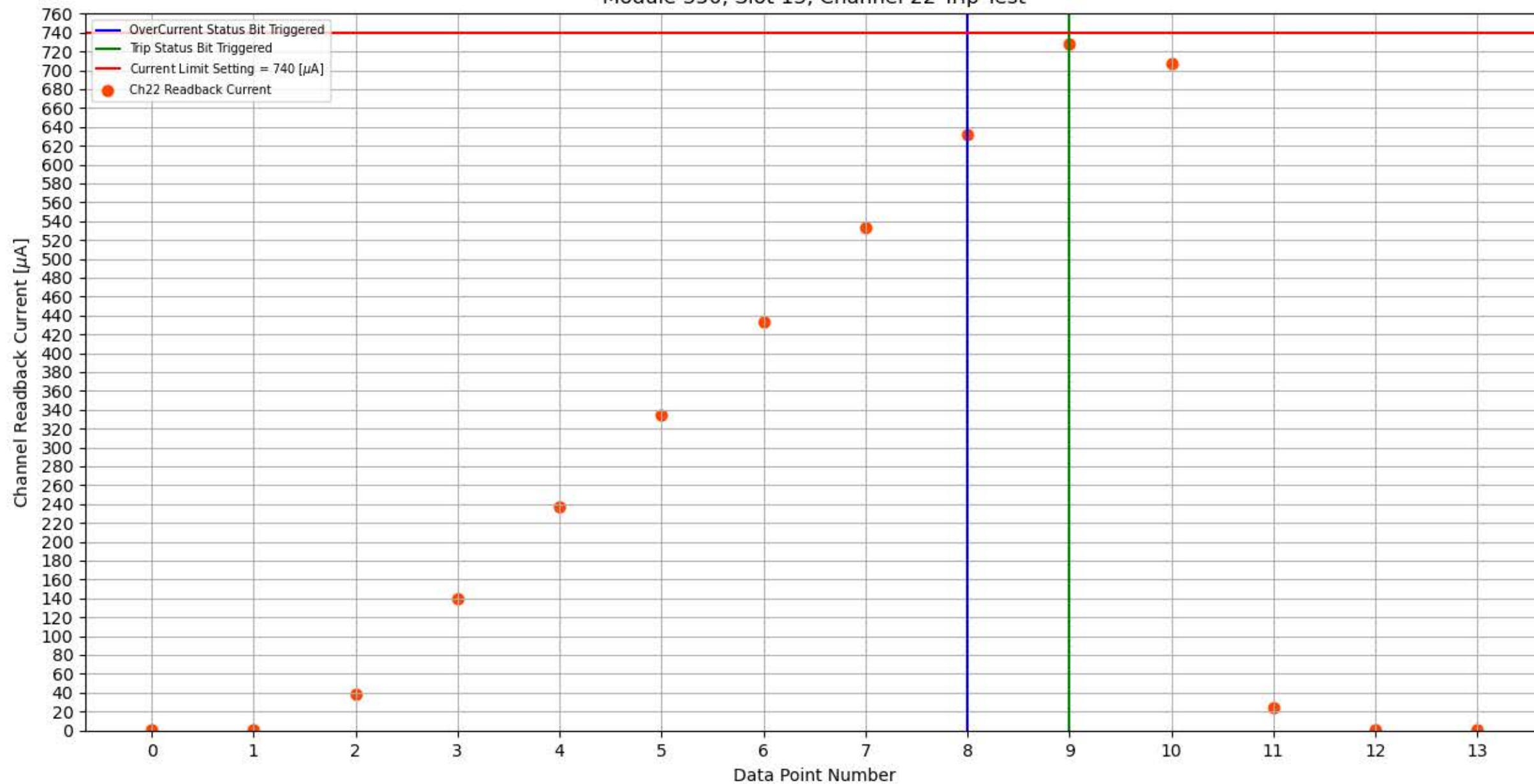
Module 350, Slot 13, Channel 22 Trip Test
