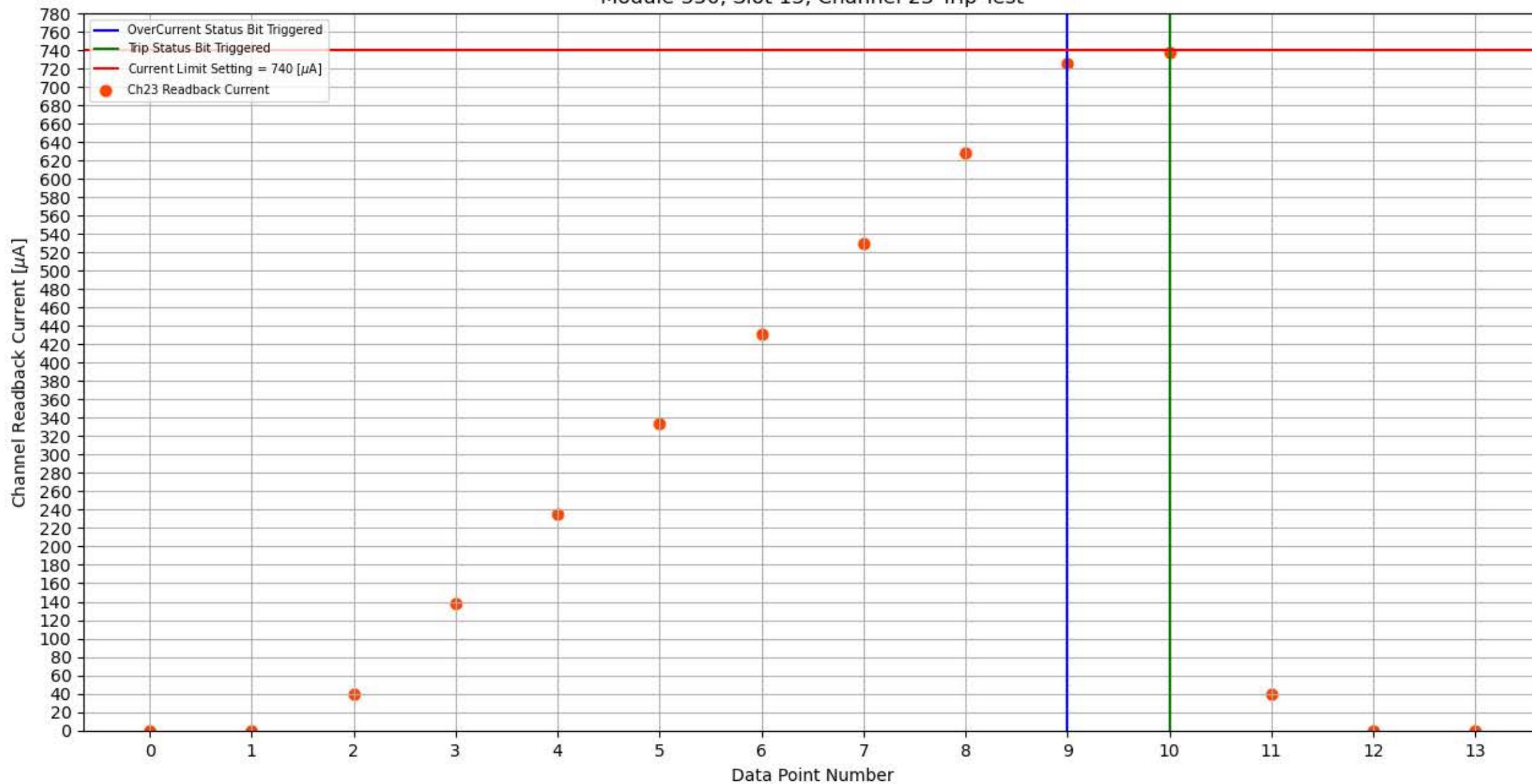
Module 350, Slot 13, Channel 23 Trip Test
