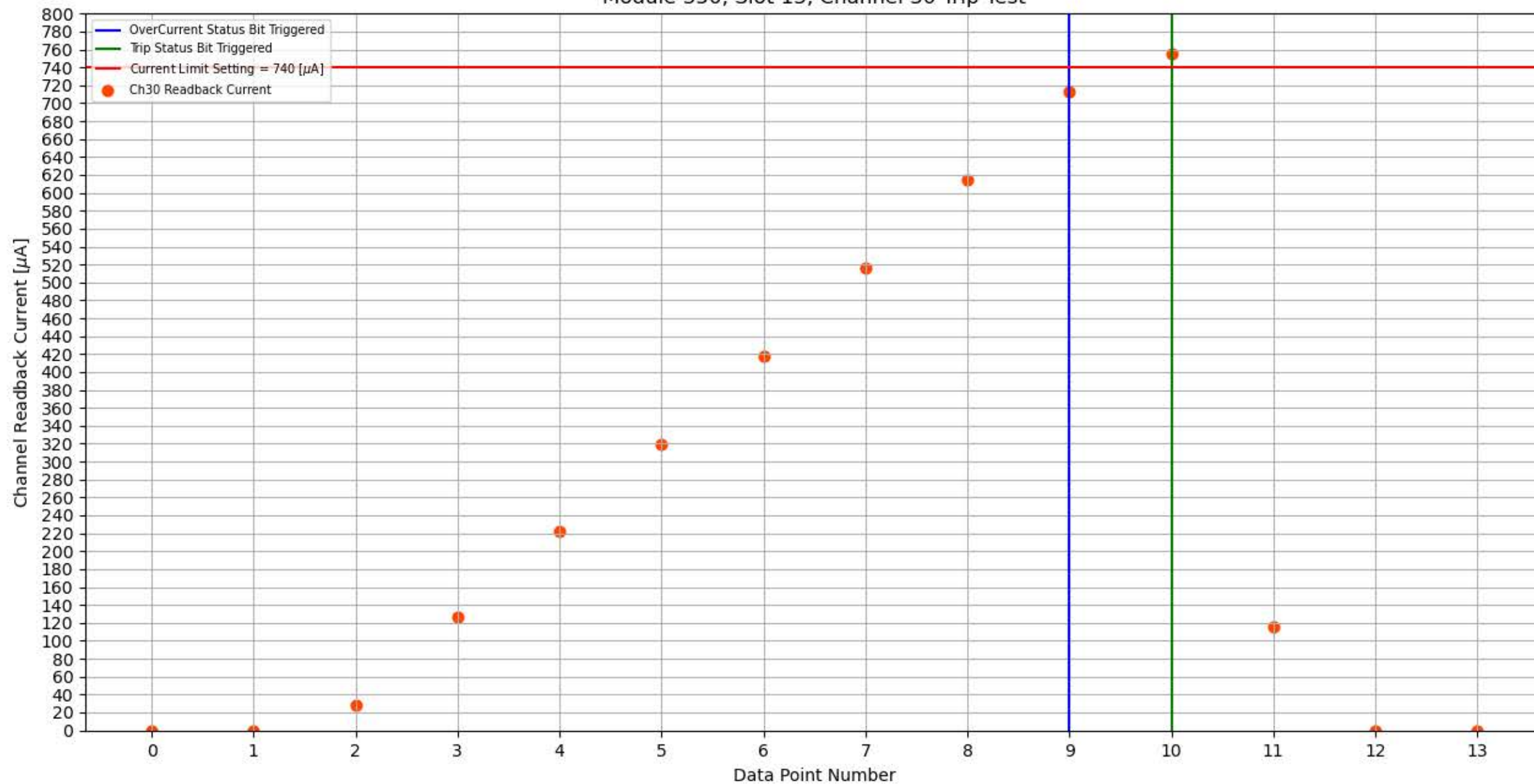
Module 350, Slot 13, Channel 30 Trip Test
