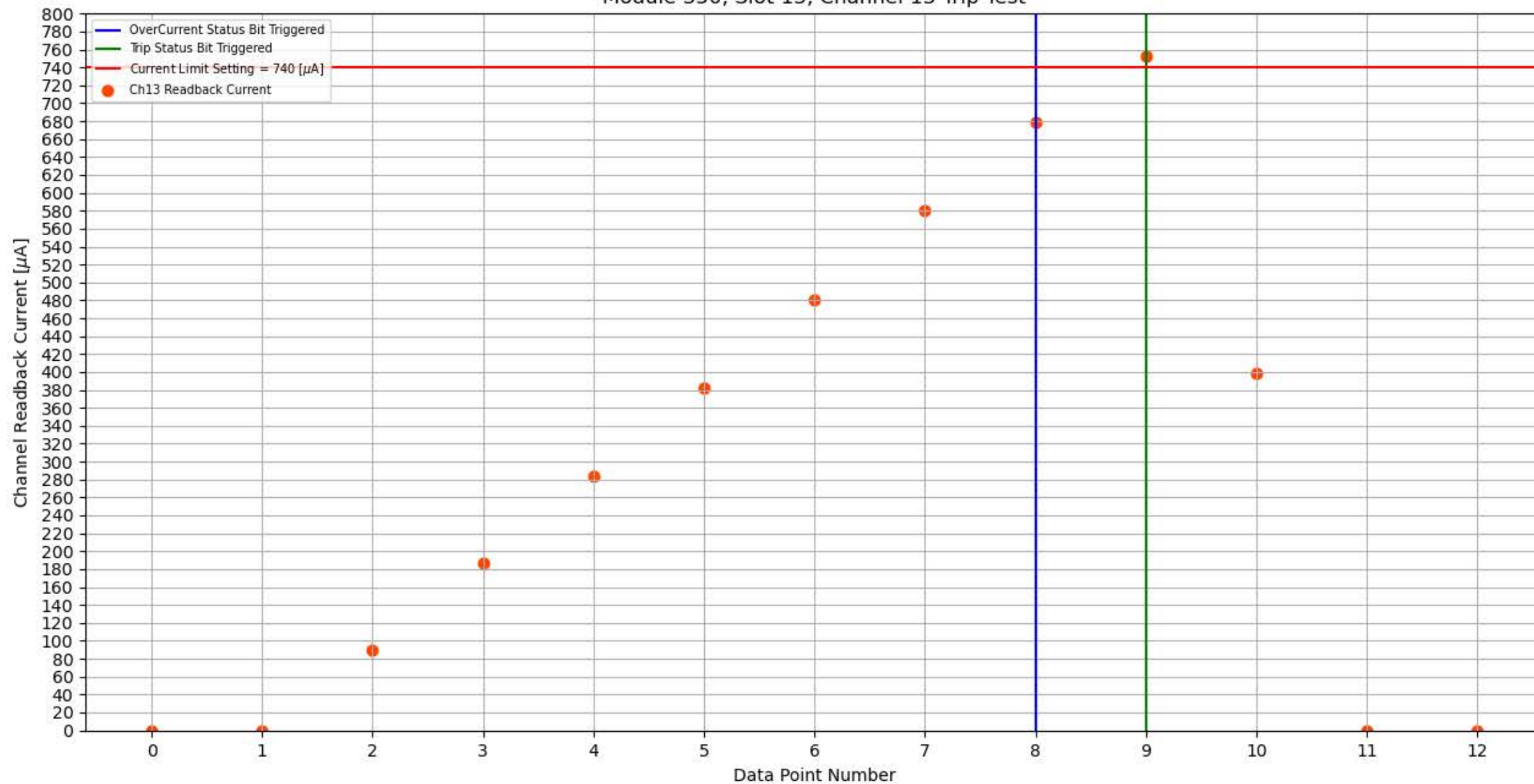
Module 350, Slot 13, Channel 13 Trip Test
