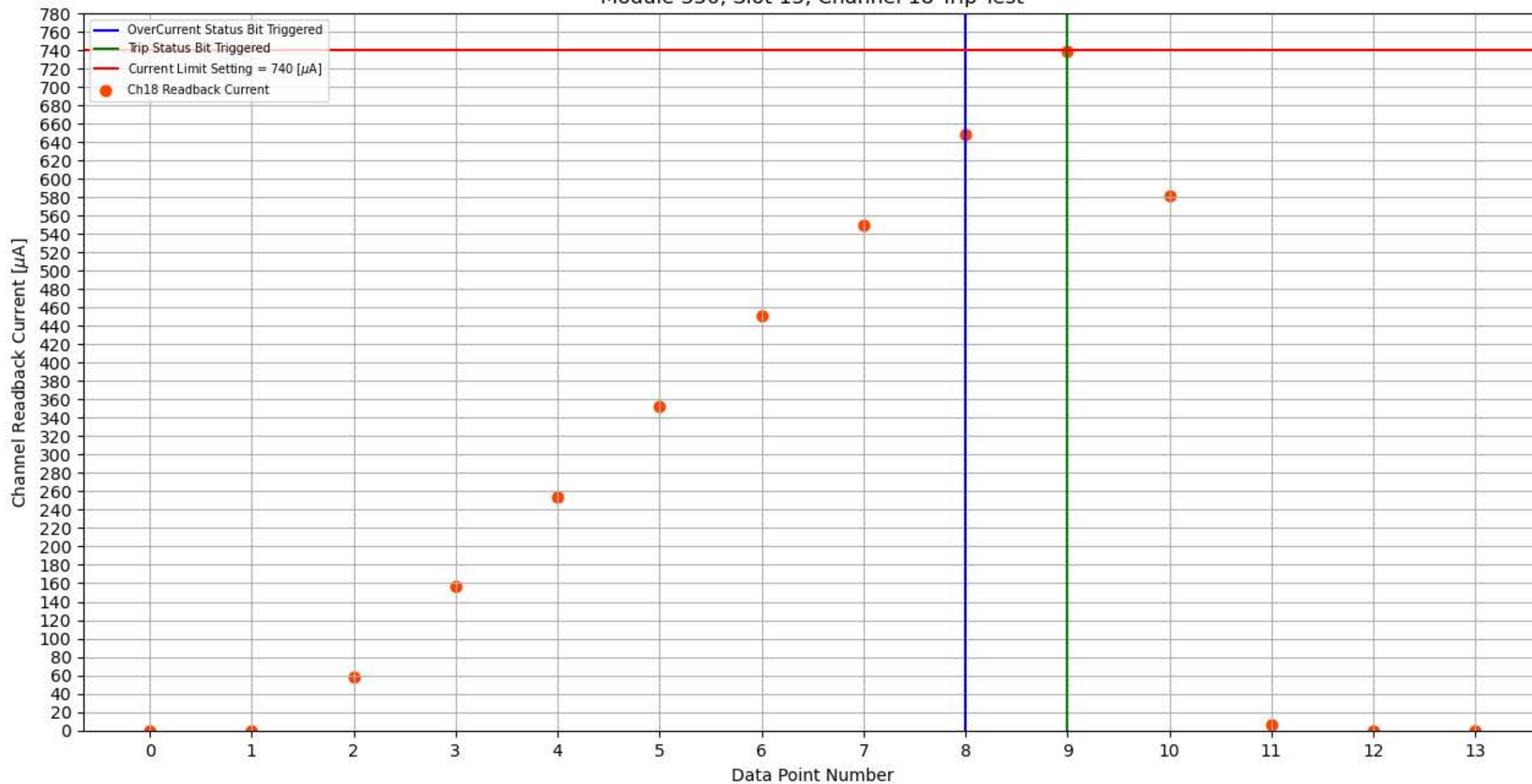
Module 350, Slot 13, Channel 18 Trip Test
