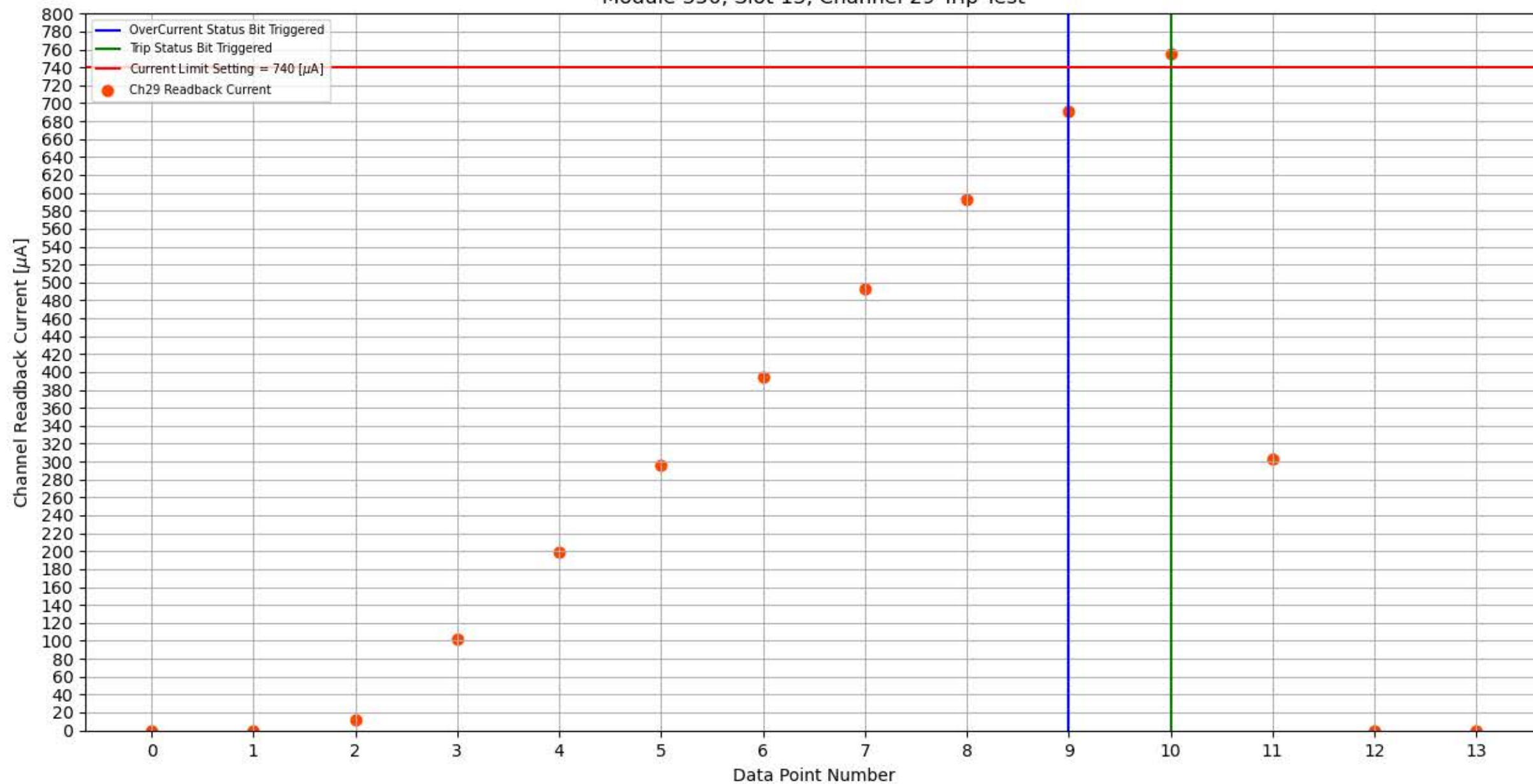
Module 350, Slot 13, Channel 29 Trip Test
