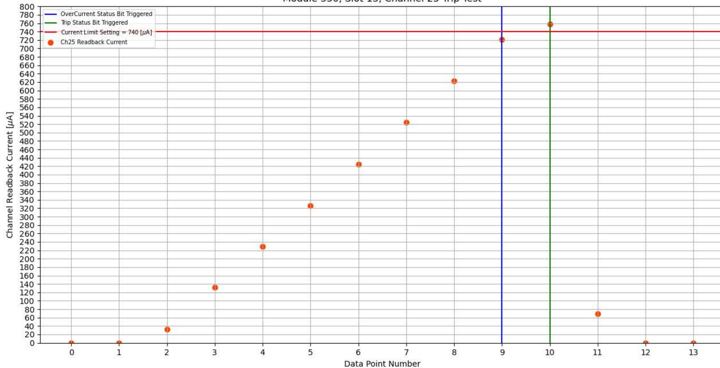
Module 350, Slot 13, Channel 25 Trip Test
