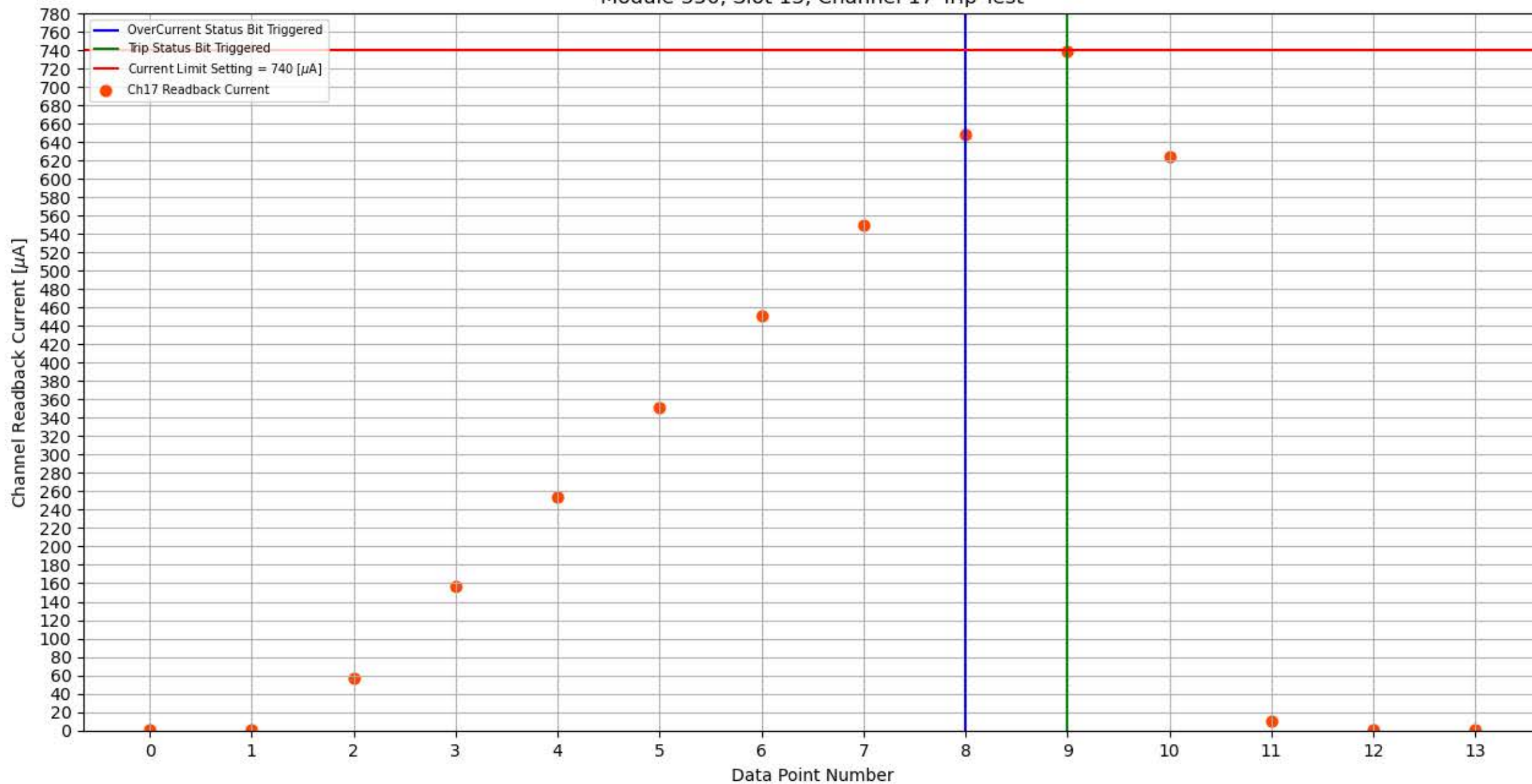
Module 350, Slot 13, Channel 17 Trip Test
