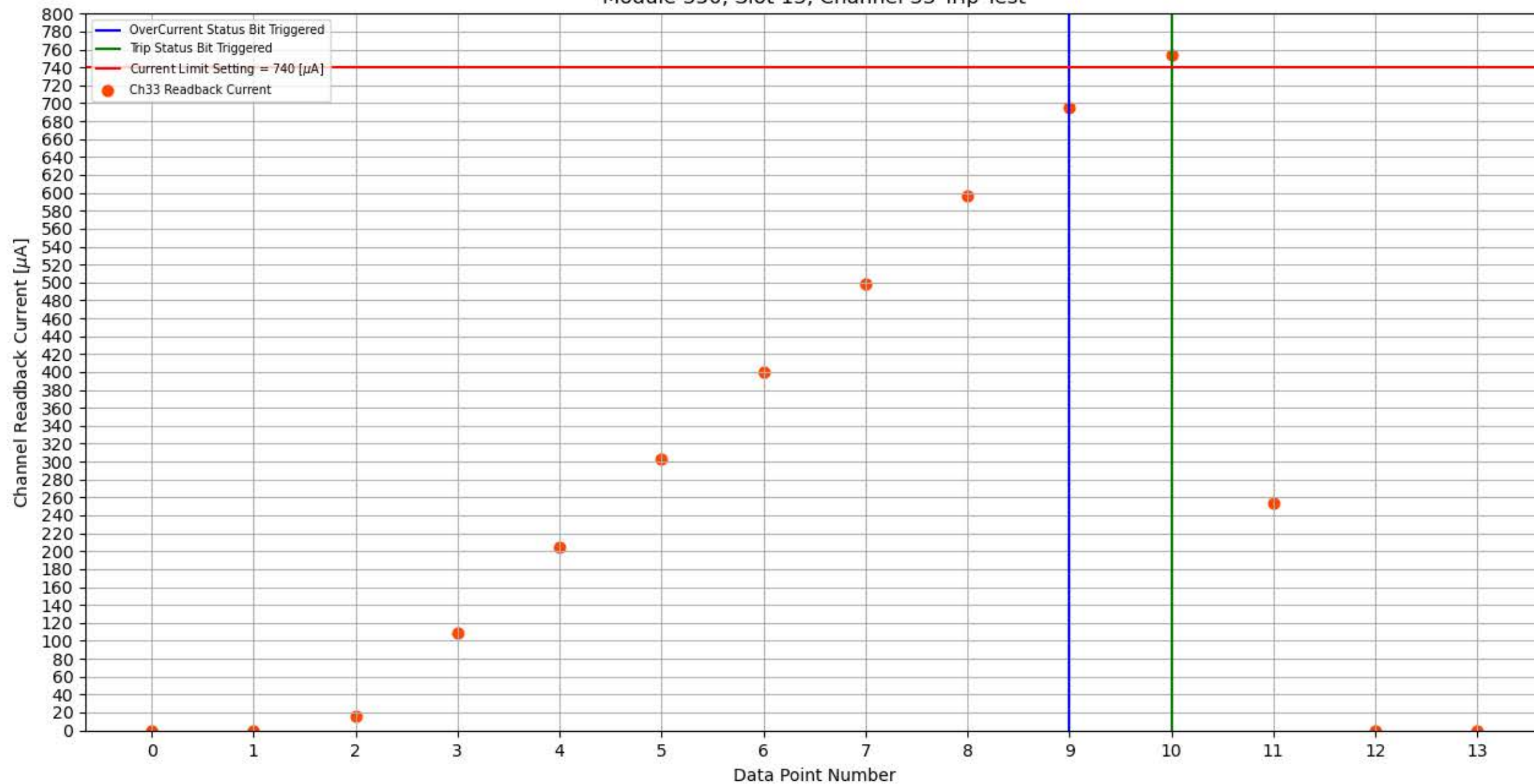
Module 350, Slot 13, Channel 33 Trip Test
