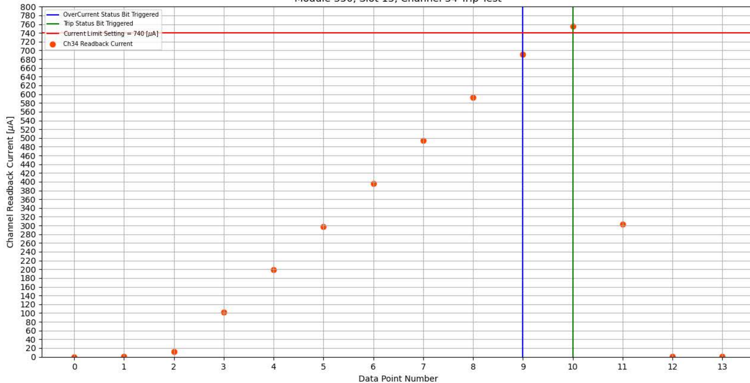
Module 350, Slot 13, Channel 34 Trip Test
